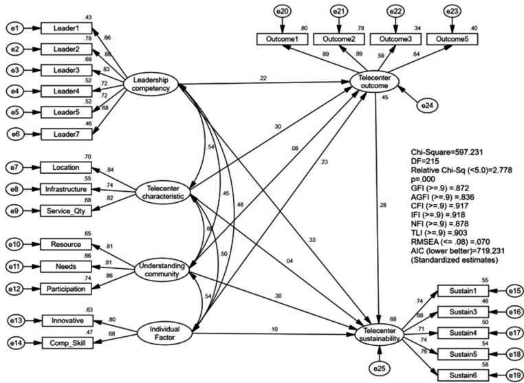
Figure 12 Structural Model
