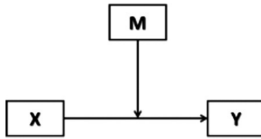
Figure 20 Moderation Effect
