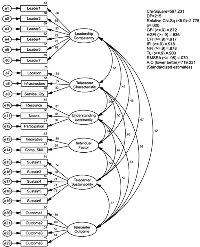
Figure 11 Measurement Model
